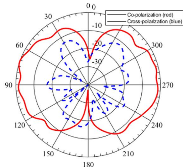
Measured Radiation pattern at 1800 MHz – 4.45 dBi
