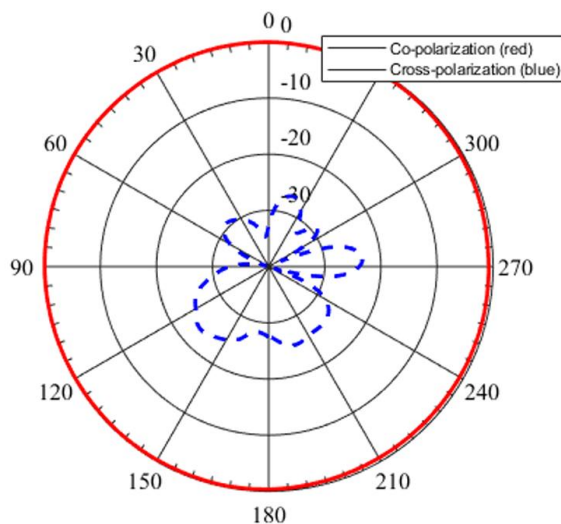
Measured Radiation pattern at 1800 MHz – 4.45 dBi
